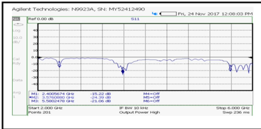
Fig 17: measured return loss of prototype antenna
