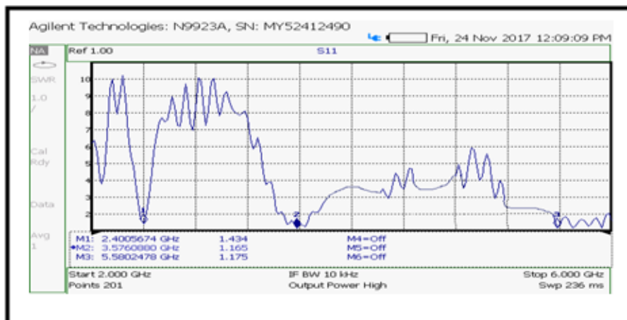
Fig 18: VSWR of measured prototype antenna
