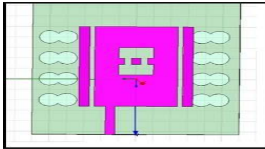
Fig 9: Modified antenna with parallel parasitic elements
