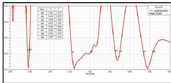
Fig 12: Bandwidth of the modified antenna
