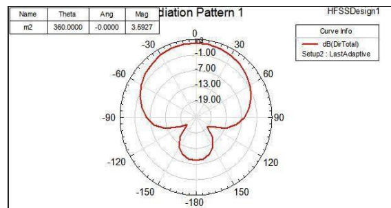
Fig 3: Radiation pattern of simple microstrip patch antenna
