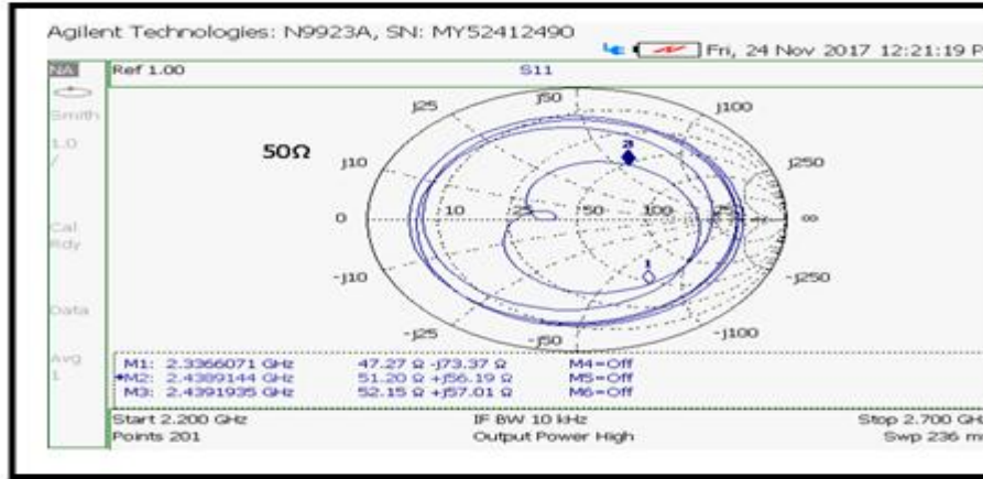
Fig 19: Impedance matching of measured prototype antenna
