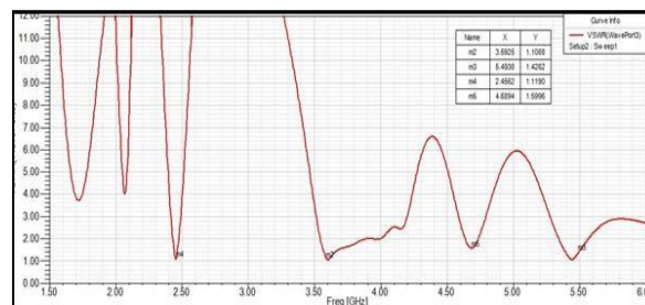
Fig 11: VSWR plot of the modified antenna
