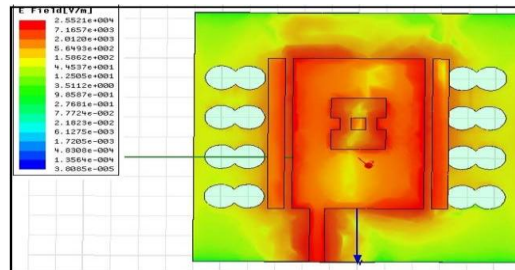
Fig 15: Current distribution in the modified antenna
