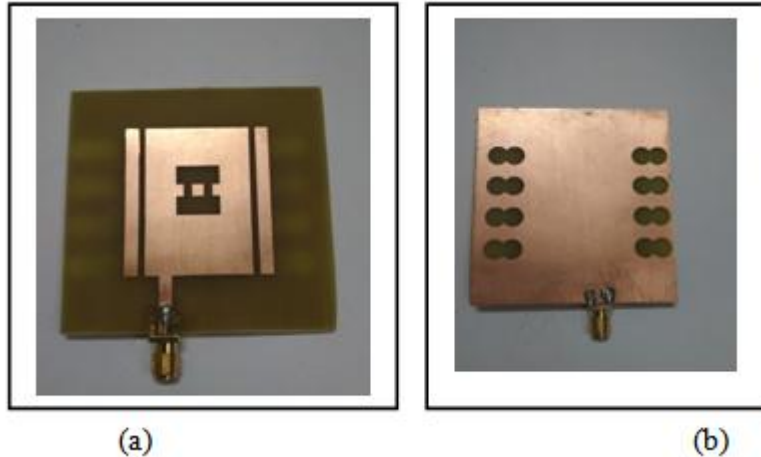
Fig 16 (a): Top view of fabricated prototype (b) Bottom view of fabricated prototype
