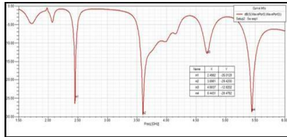
Fig 10: Simulated S11 plot of the modified antenna
